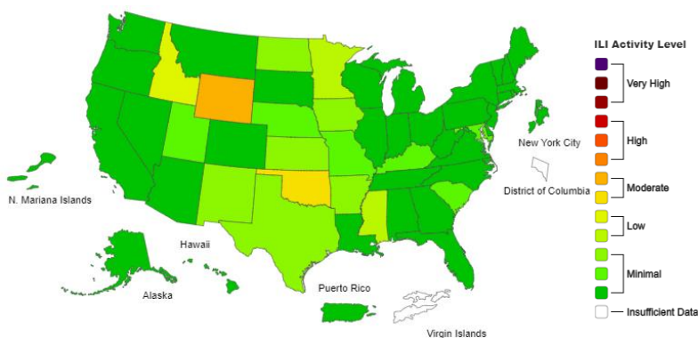
Figure 1a. National ILI Activity Level Map from CDC, week 7
