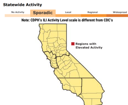
Figure 1b. State ILI Activity Level Map from CDPH, week 7
